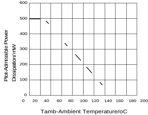
Figure 2. Power De-rating
